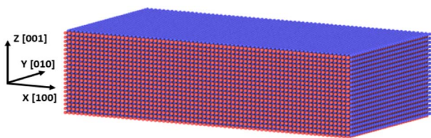
Fig. 1. Bulk B2–CuZr with periodic boundary conditions.
